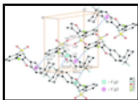
Fig. 2. A view of the C—H...O and C—H... \pi interactions (dotted lines) in the crystal structure of the title compound. [Symmetry codes: (i) -x + 1, -y + 1, -z + 1 ; (ii) -x + 1, -y + 2, -z + 1 ; (iii) x + 1, y, z .]
